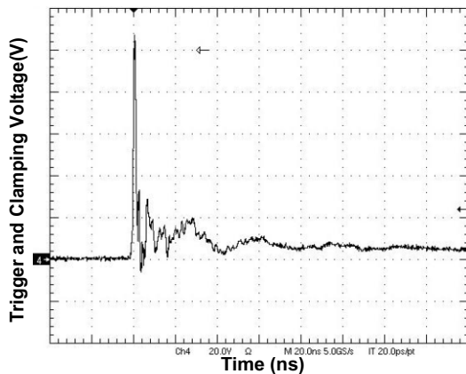
Fig.5 IEC61000-4-2 +8kV Contact Discharge
